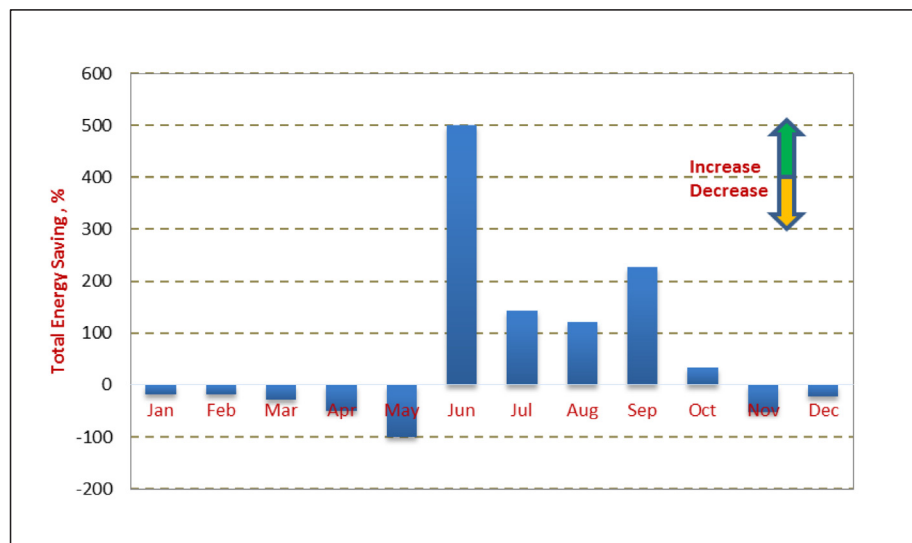
Fig. 10. Total energy saving in the case of with atrium on monthly basis.
