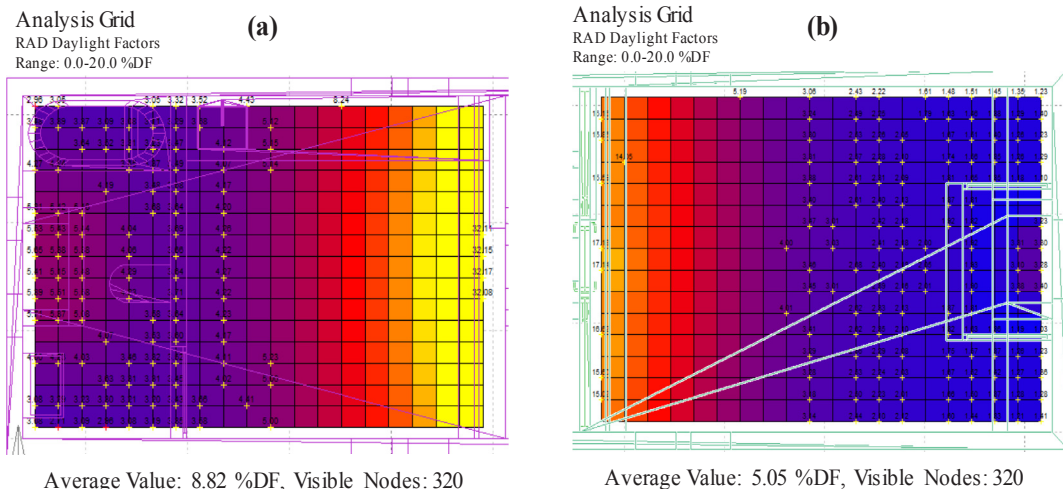
Fig. 6. The distribution of DF at the height of 800 mm above the first floor; (a) Behind the building, (b) Front of the building.
