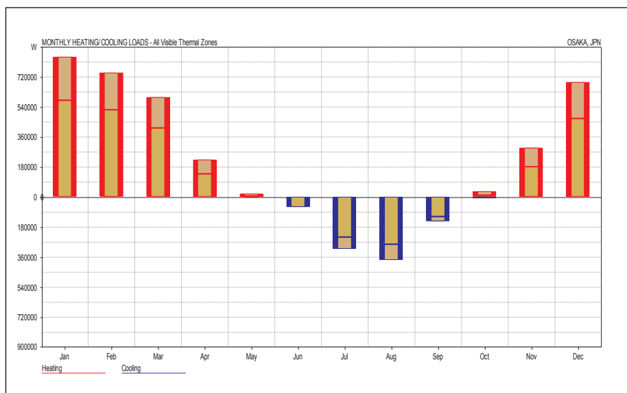
Fig. 9. Annual heating and cooling energy demand with an atrium.
